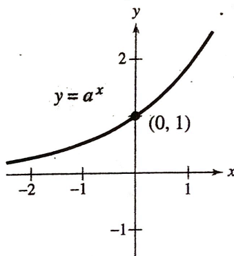
Exponential Function
