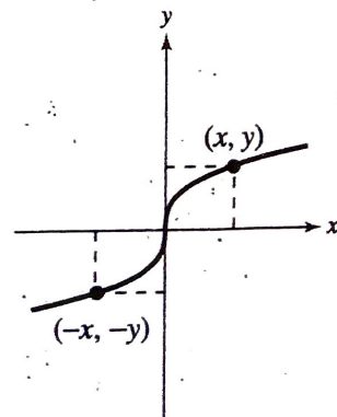
Origin Symmetry
