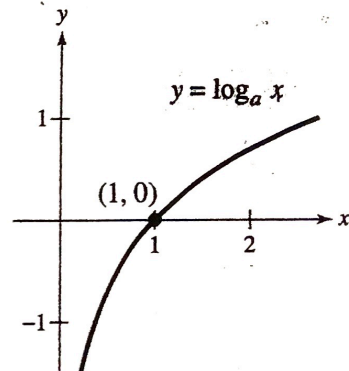
Logarithmic Function
