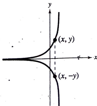
x-Axis Symmetry
