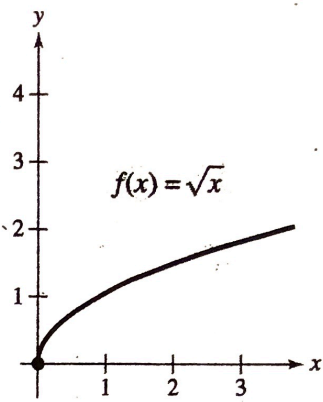
Square Root Function
