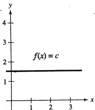
Constant Function
