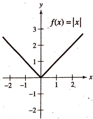
Absolute Value Function
