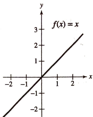
Identity Function
