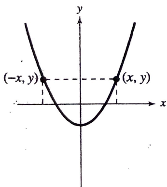
y-Axis Symmetry
